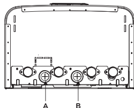
(Pro Hydrosplit)
