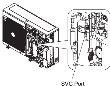
SVC Port
